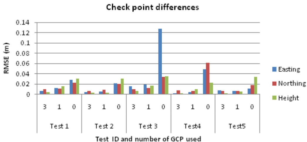
Figure 5: Results of bundle adjustments using directly determined exterior orientation data. For each data set bundle adjustment was done three times varying the number of control points (3, 1, and 0 control points).
